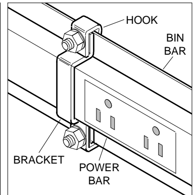
Figure 4-Bracket Detail
