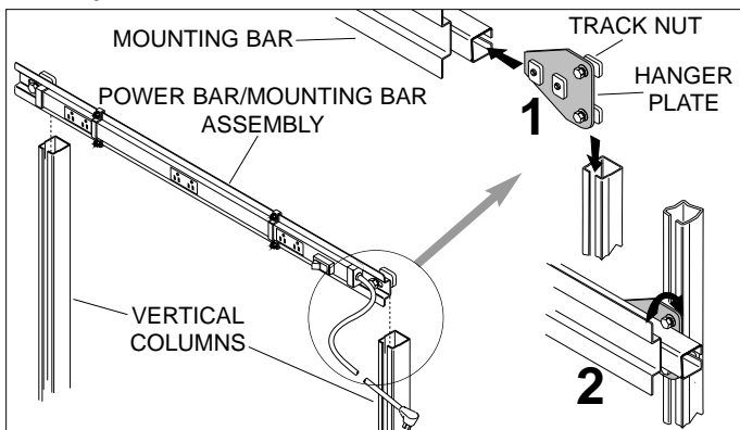
Figure 2-Support Bar Installation
