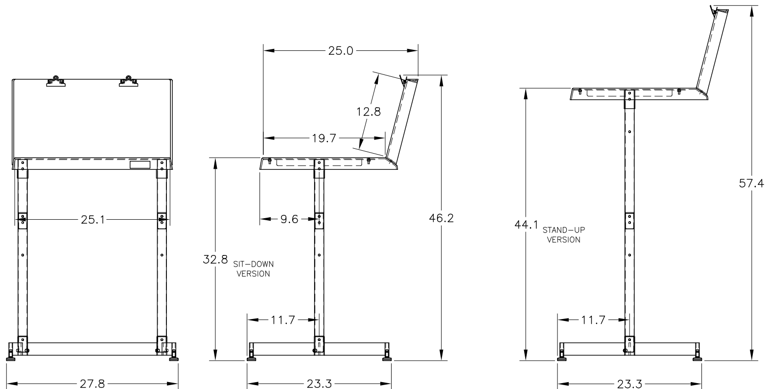
GENERAL DIMENSIONAL DRAWING QUALTECH A2700S DOCUMENT STAND
