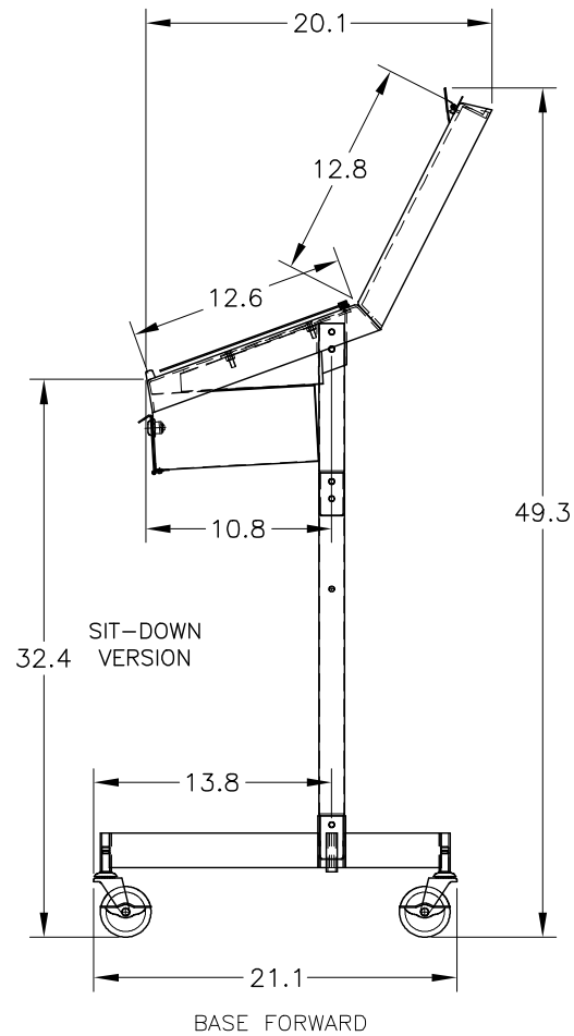
GENERAL DIMENSIONAL DRAWING QUALTECH A1000D DOCUMENT STAND
