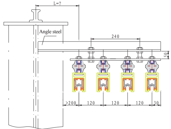
Method three: This mounting method is applicable for high voltage (3kV and below) and outdoor insulated aluminum bar enclosures.
