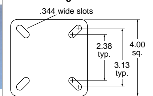
Post Mounting Base Dimensions
